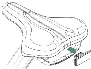
Figure 2 - Remove reflector.
