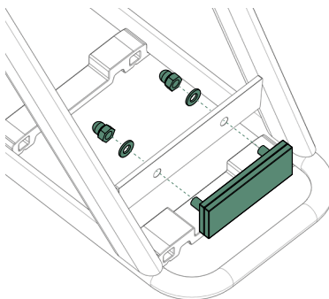
Figure 3 - Mount reflector.
