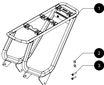
Figure 1 - Lovens Explorer 2 rear carrier parts.
