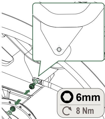
Figure 6 - Aligning rear mounting points.
